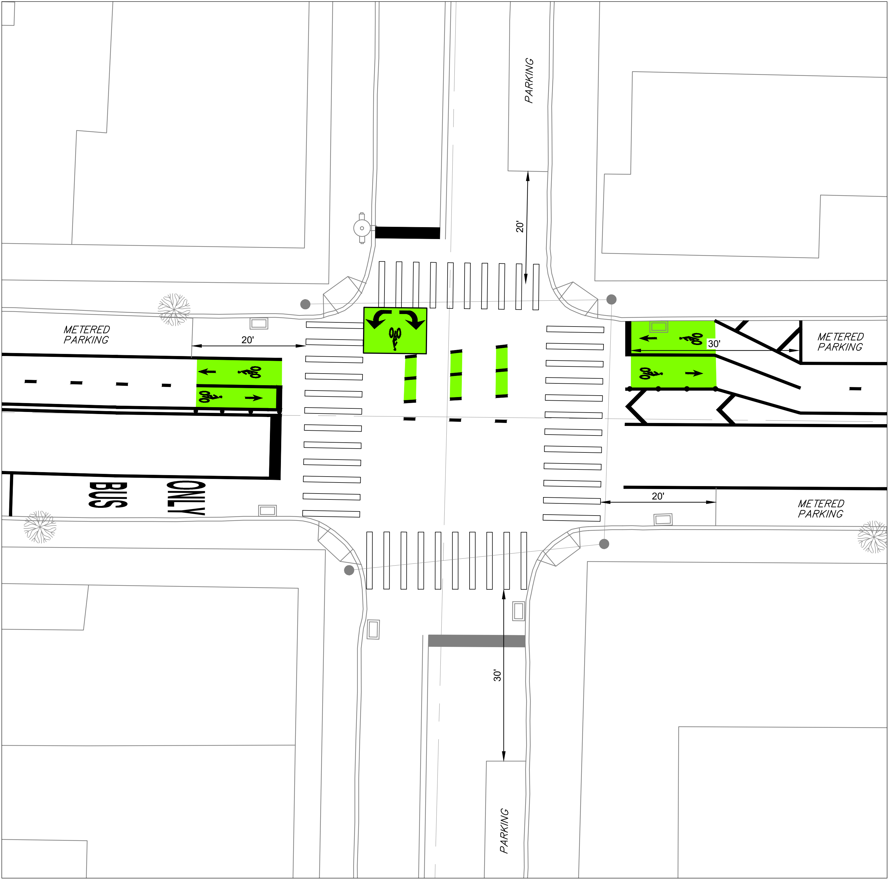
TYPICAL CYCLE TRACK INTERSECTION MARKINGS DETAIL SCALE: 1"=10'
