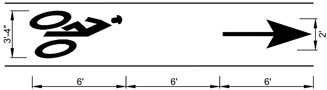
TYPICAL BIKE LANE MARKING DETAIL N.T.S.
