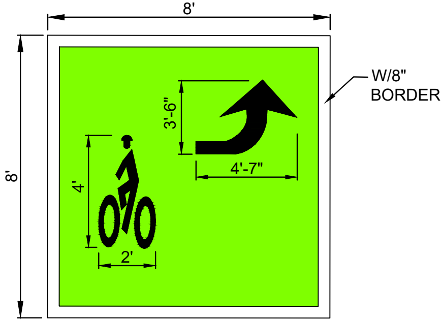
BICYCLE TURN QUEUE BOX W/ GREEN BACKGROUND DETAIL N.T.S.
