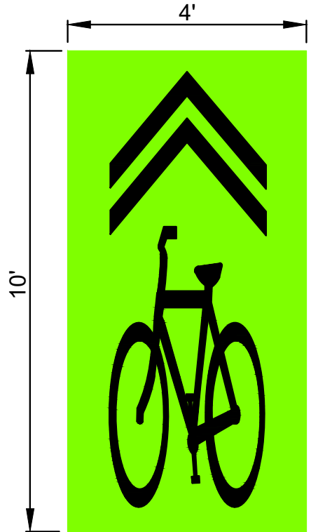
SHARED LANE ARROW MARKING "SHARROW" W/ GREEN BACKGROUND DETAIL N.T.S.
