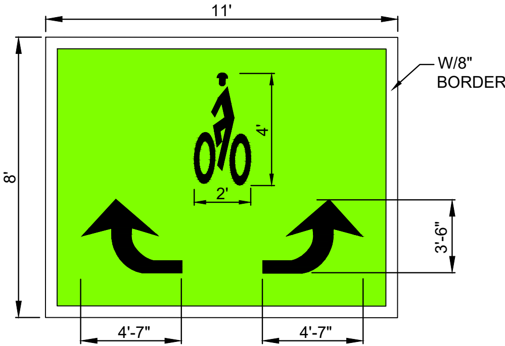
BICYCLE TURN 2 STAGE QUEUE BOX W/ GREEN BACKGROUND DETAIL N.T.S.
