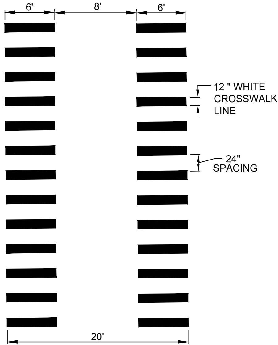
RAIL TRAIL CROSSWALK MARKINGS DETAIL N.T.S.
