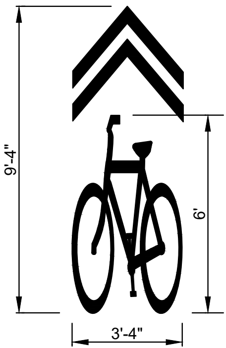
TYPICAL SHARED LANE ARROW MARKING "SHARROW" DETAIL PENNDOT PUB. 111M N.T.S.
