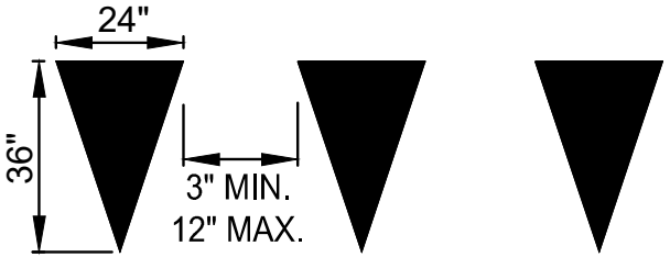
LARGE YIELD LINE DETAIL N.T.S.
