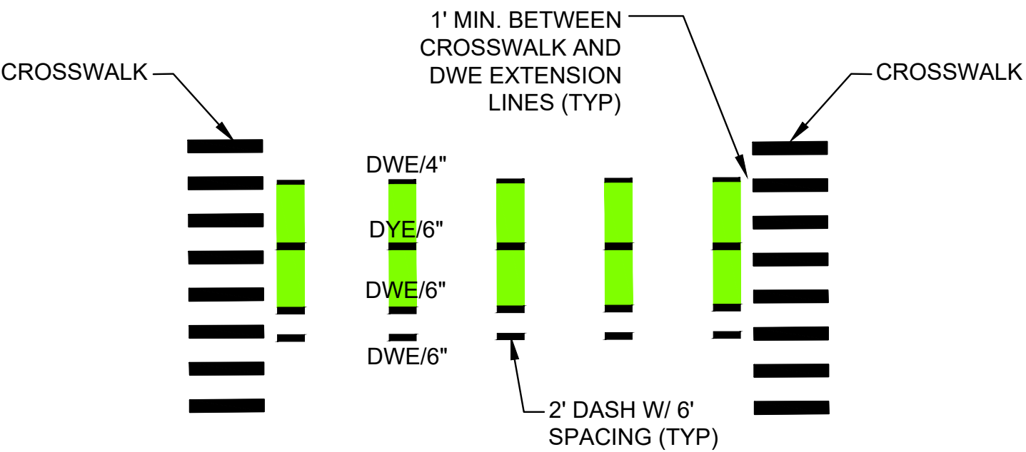
TYPICAL CYCLE TRACK INTERSECTION EXTENSION MARKINGS W/ GREEN BACKGROUND DETAIL N.T.S.
