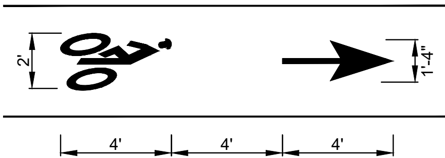
CYCLE TRACK BIKE LANE MARKING DETAIL N.T.S.
