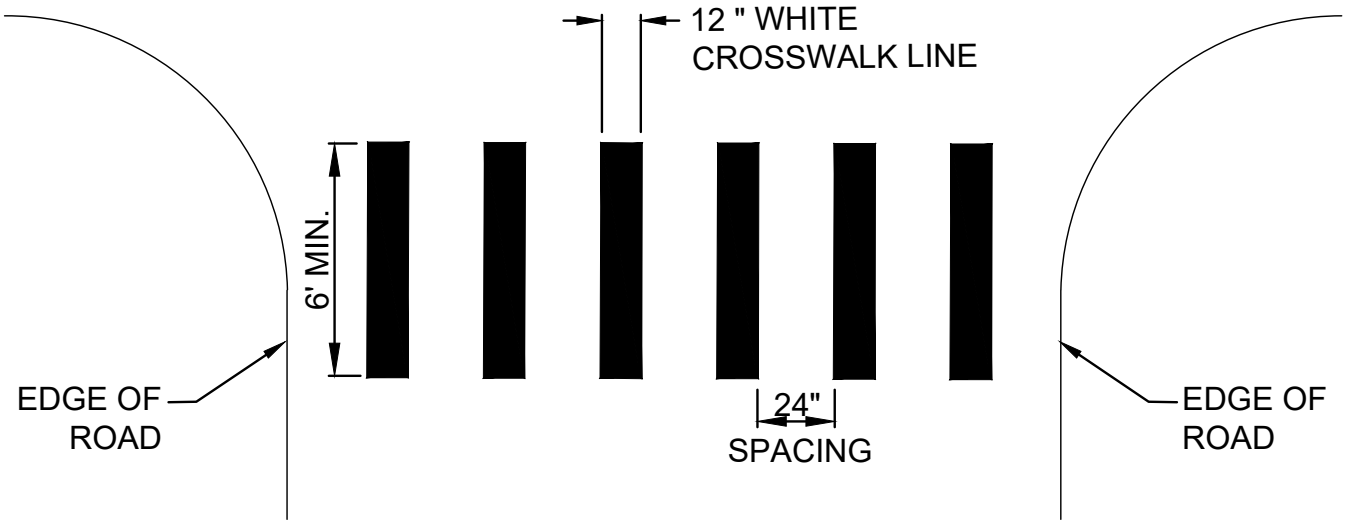
HIGH VISIBILITY PIANO KEY CROSSWALK MARKINGS N.T.S.
