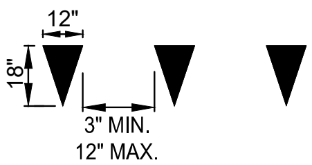
SMALL YIELD LINE DETAIL N.T.S.
