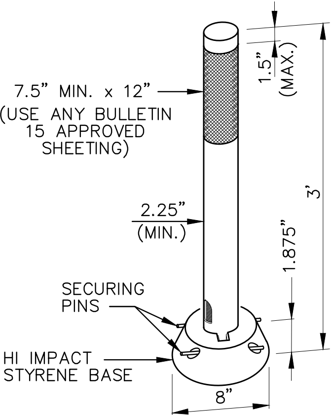
TYPE SM-1 SURFACE-MOUNTED POSTS N.T.S.
